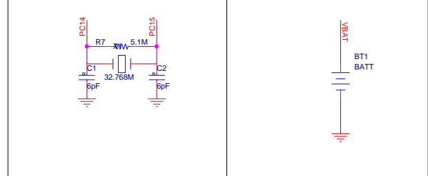
RTC CLOCK
