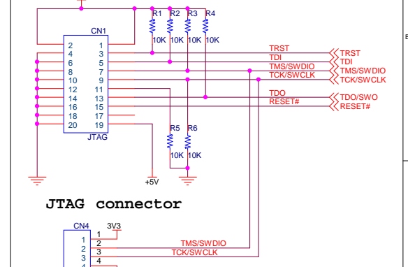
SWD Download/Dubeg connectors
